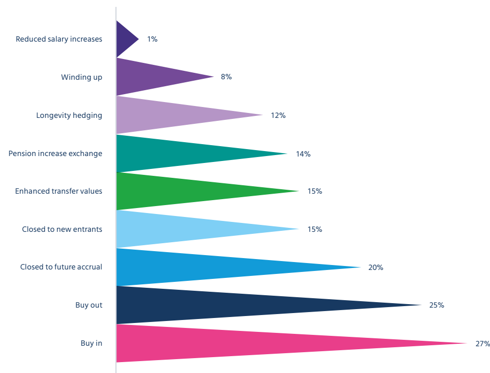
Figure 20. Proportion of plans considering risk-management exercises over the last year
